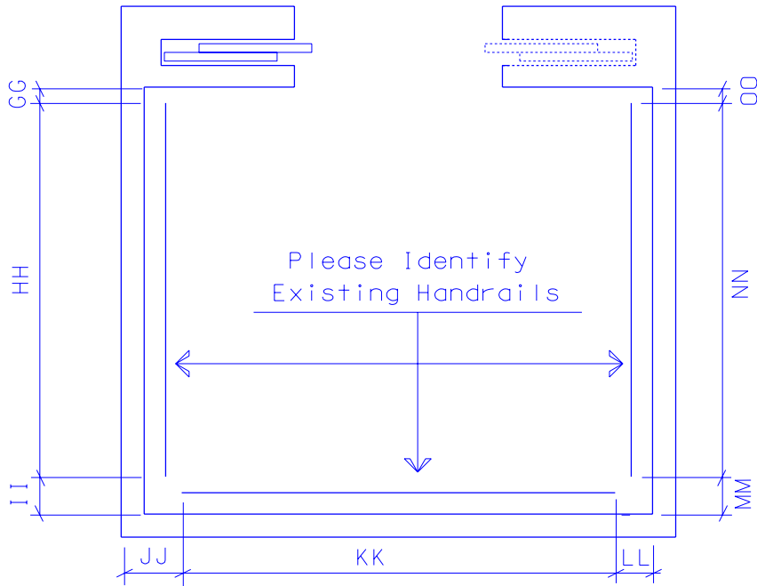
CAB HANDRAILS
